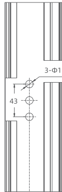
有底座执手+传动锁盒开孔尺寸 With Base Handle+ Dimension Of Screw Hole Trepanning
