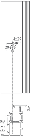
无底座执手+传动锁盒开孔尺寸 Non-plus Handle + Dimension Of Screw Hole Trepanning
