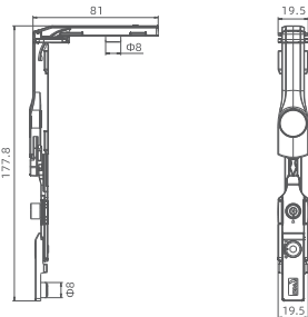
Adjustable Corner Drive With Mishandling Device And Locking Cam 可调偏轴钉转角器（含防误操作）
