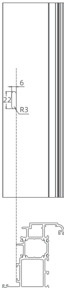
免铣槽执手+传动锁盒开孔尺寸 Unnecessary Groove Milling Handle + Dimension Of Screw Hole Trepanning
