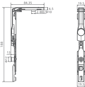
Adjustable Corner Drive With Mishandling Device And Mushroom Cam 可调防撬转角器（含防误操作）
