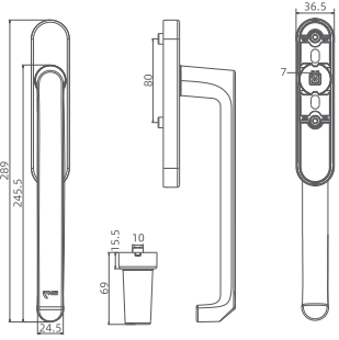
Parallel Retraction Sliding Door Handle Without Keyhole (Exterior) 侧压推拉门执手不带锁孔（室外侧）
