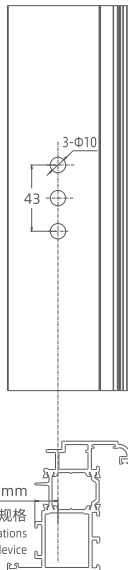
有底座执手+传动锁盒开孔尺寸 With Base Handle + Dimension Of Screw Hole Trepanning
