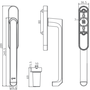
Parallel Retraction Sliding Door Handle Without Keyhole (Interior) 侧压推拉门执手不带锁孔（室内侧）
