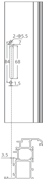
拨叉执手+连接块开孔尺寸 Fork Handle + Dimension Of Screw Hole Trepanning
